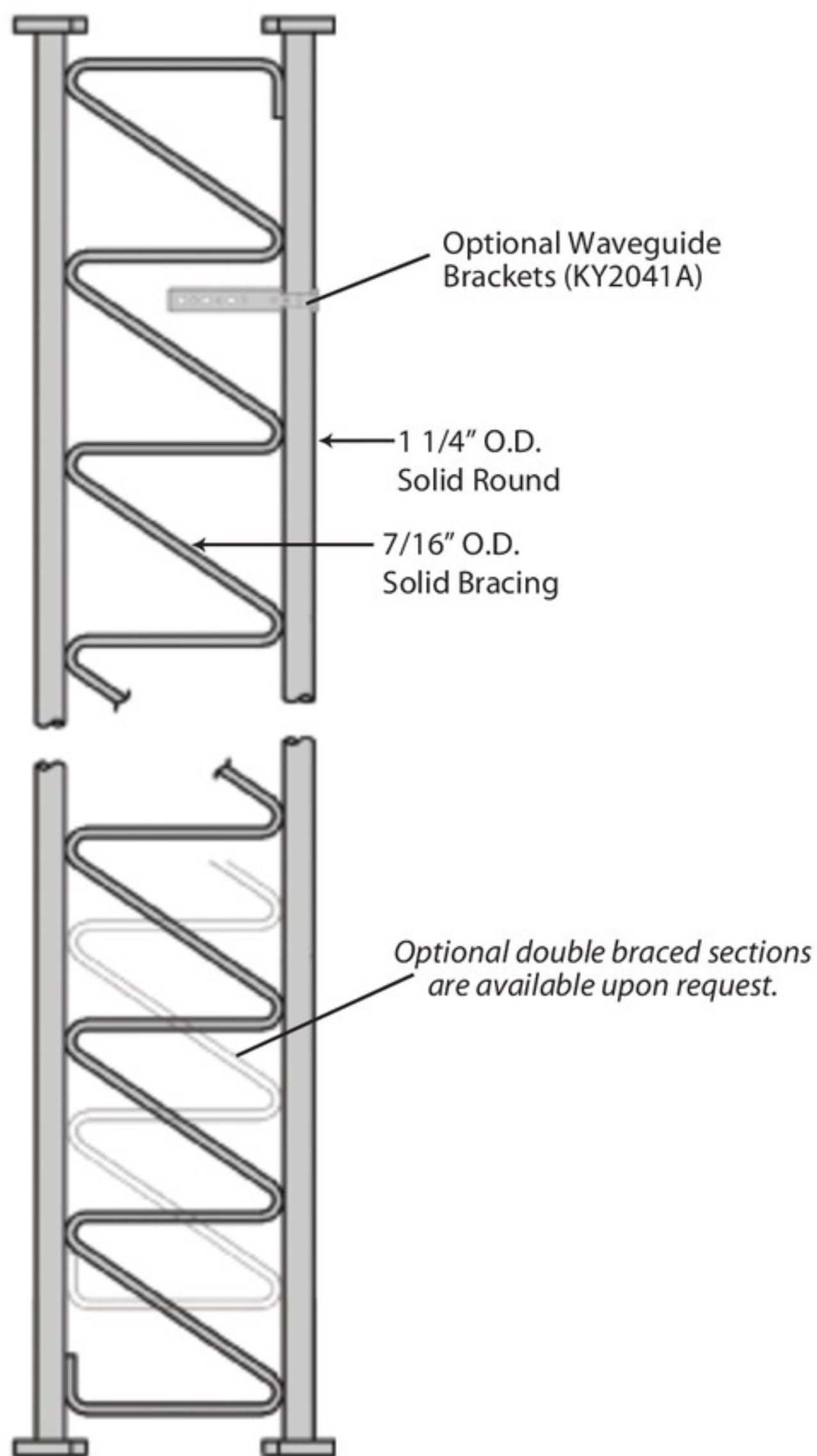
STANDARD SECTION 45GSR10 - 10' Section 45GSR20 - 20' Section
