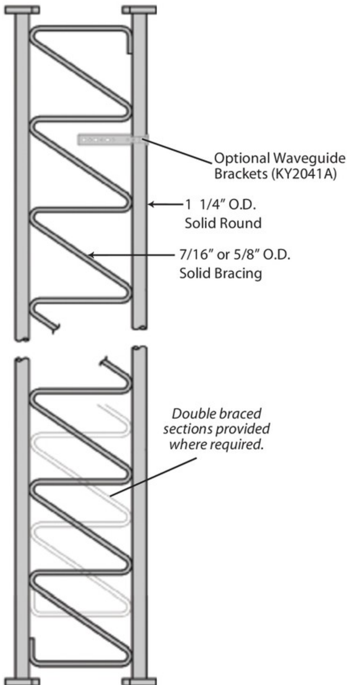
STANDARD SECTION 45GSR10 - 10' Section 45GSR20 - 20' Section
