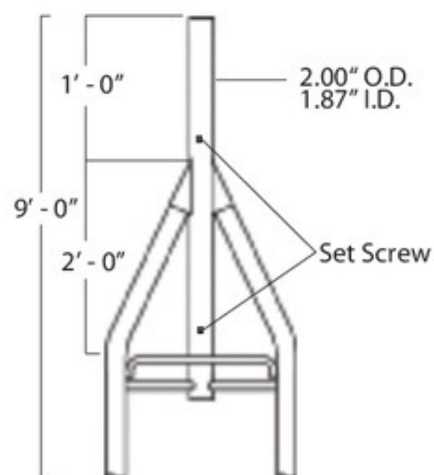
TOP SECTION 45AG
