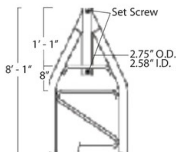
TOP SECTION 45AG5
