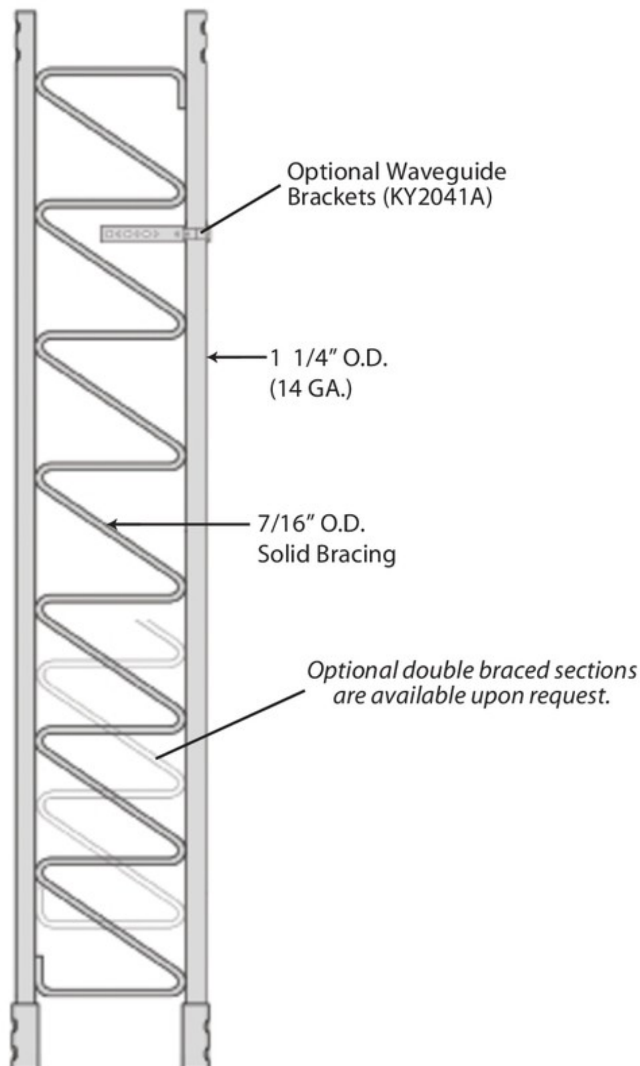
STANDARD SECTION 45G - 10' Section
