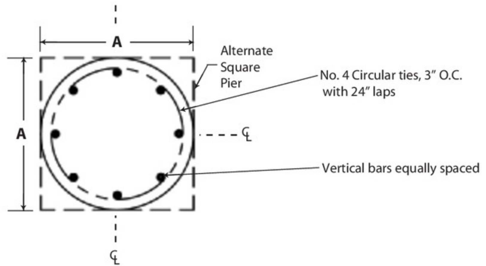
PLAN VIEW
