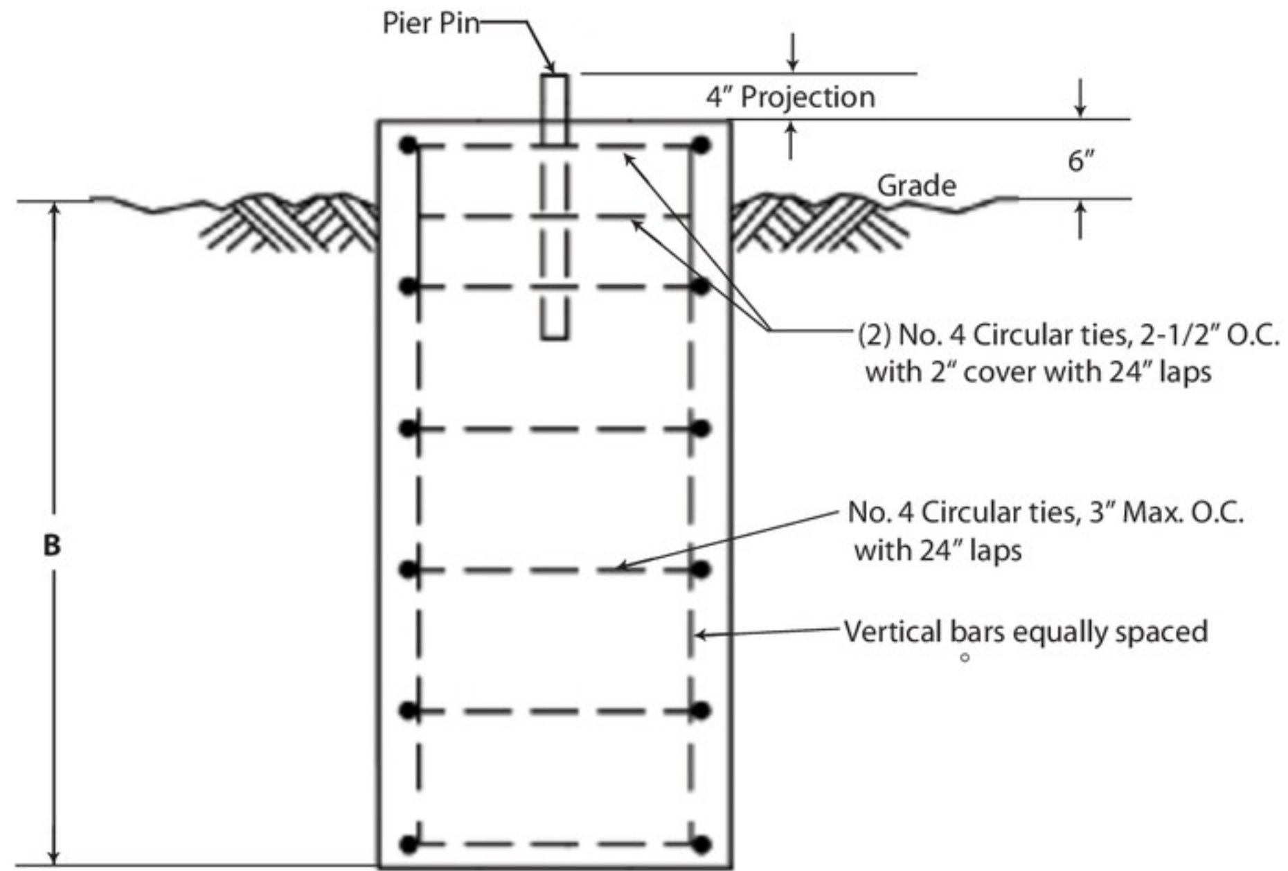
ELEVATION VIEW
