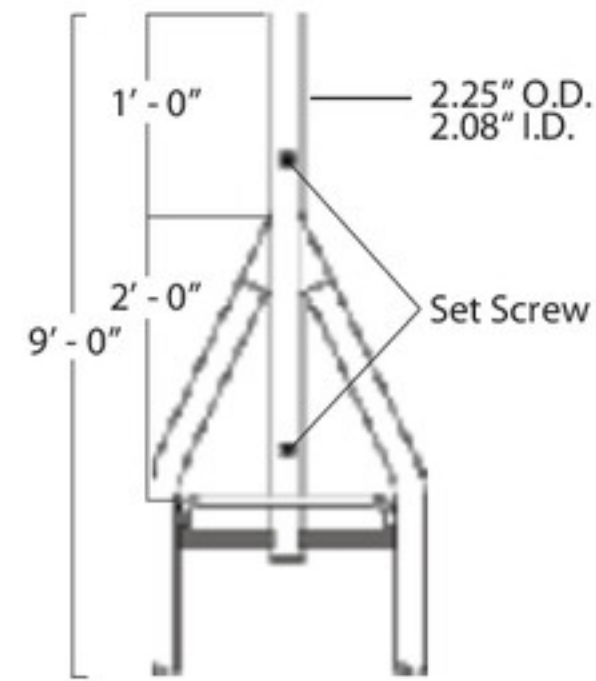
TOP SECTION 45AG3
