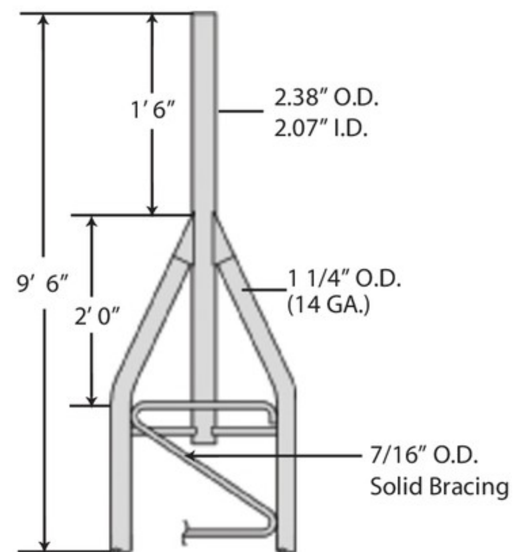
STANDARD TOP SECTION 45AG2
