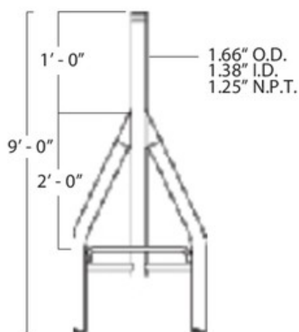
TOP SECTION 45AG1
